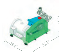
HIGH PRESSURE PUMP
